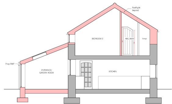
Section B-B, 1:50
